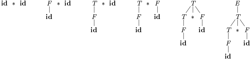
Figure 4.25: A bottom-up parse for \mathbf{id * id}
